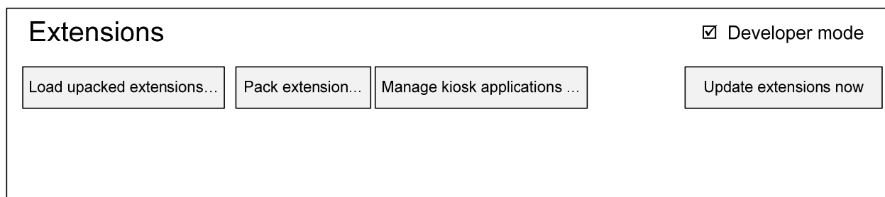
Figure 12. Extensions Screen
